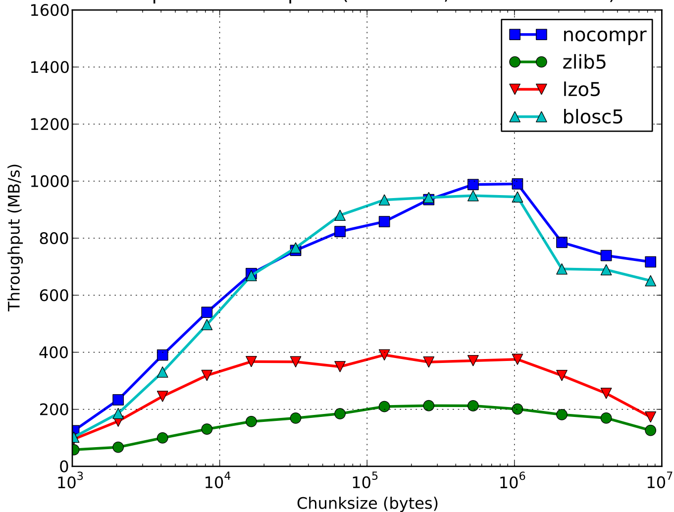
Sequential read speed (2 GB data, 8 MB cache size)
