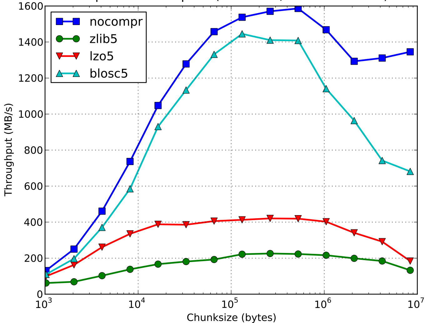
Sequential read speed (2 GB data, 1 MB cache size)
