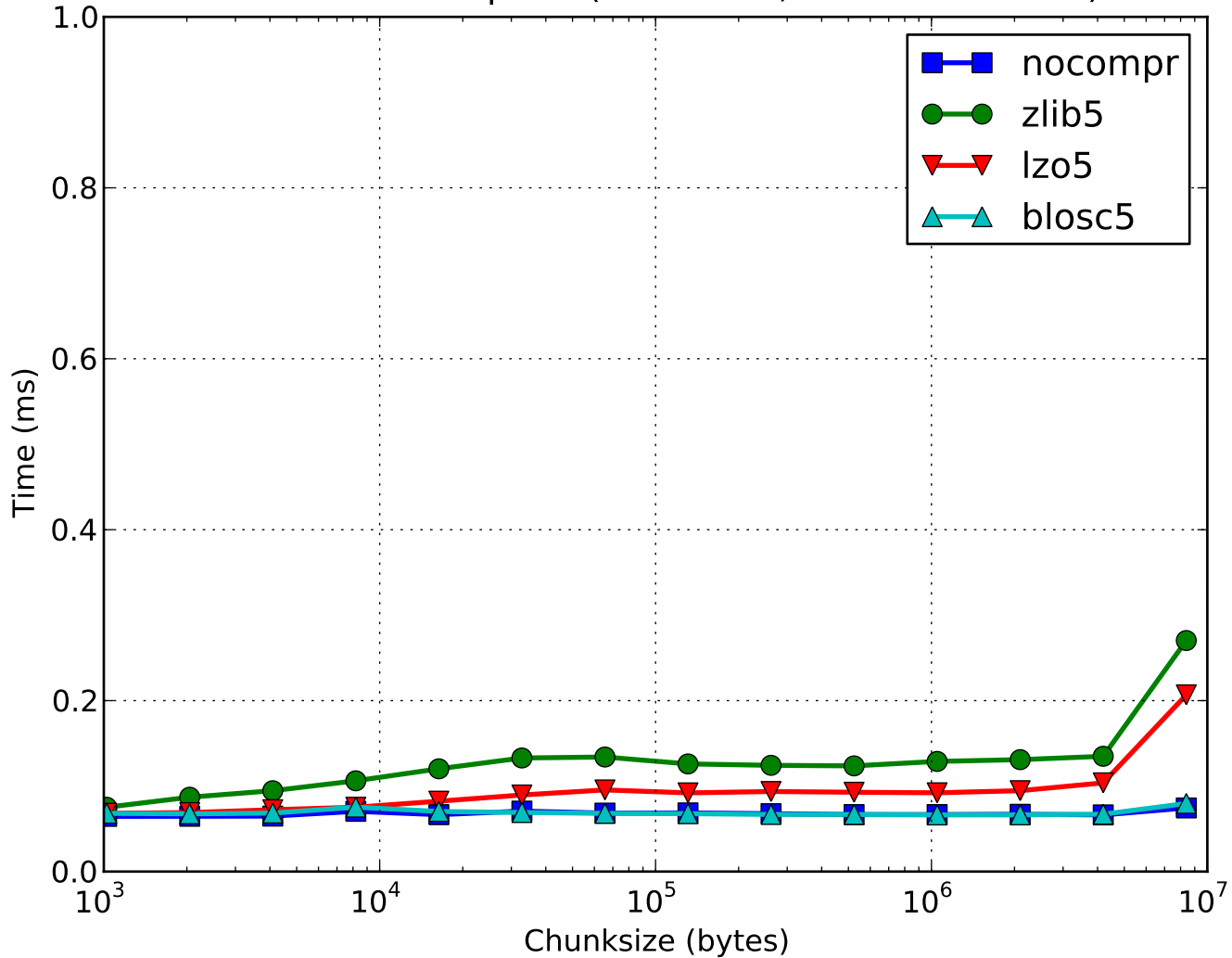
Random read speed (2 GB data, 8 MB cache size)
